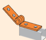
Hinged Bracket
